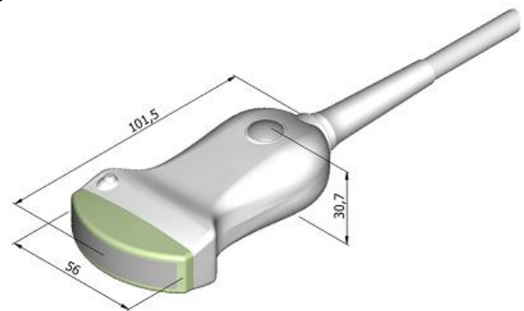
Fig. 1 9C2 transducer
